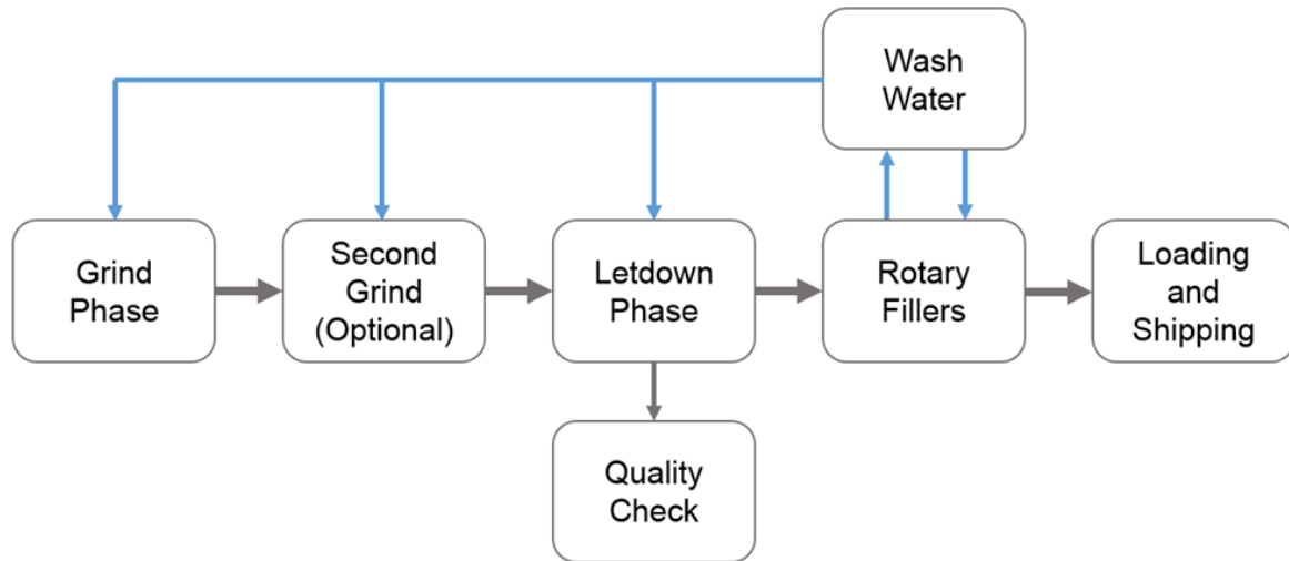
Figure 2: Behr Process and Masterchem Industries LLC process flow schematic
